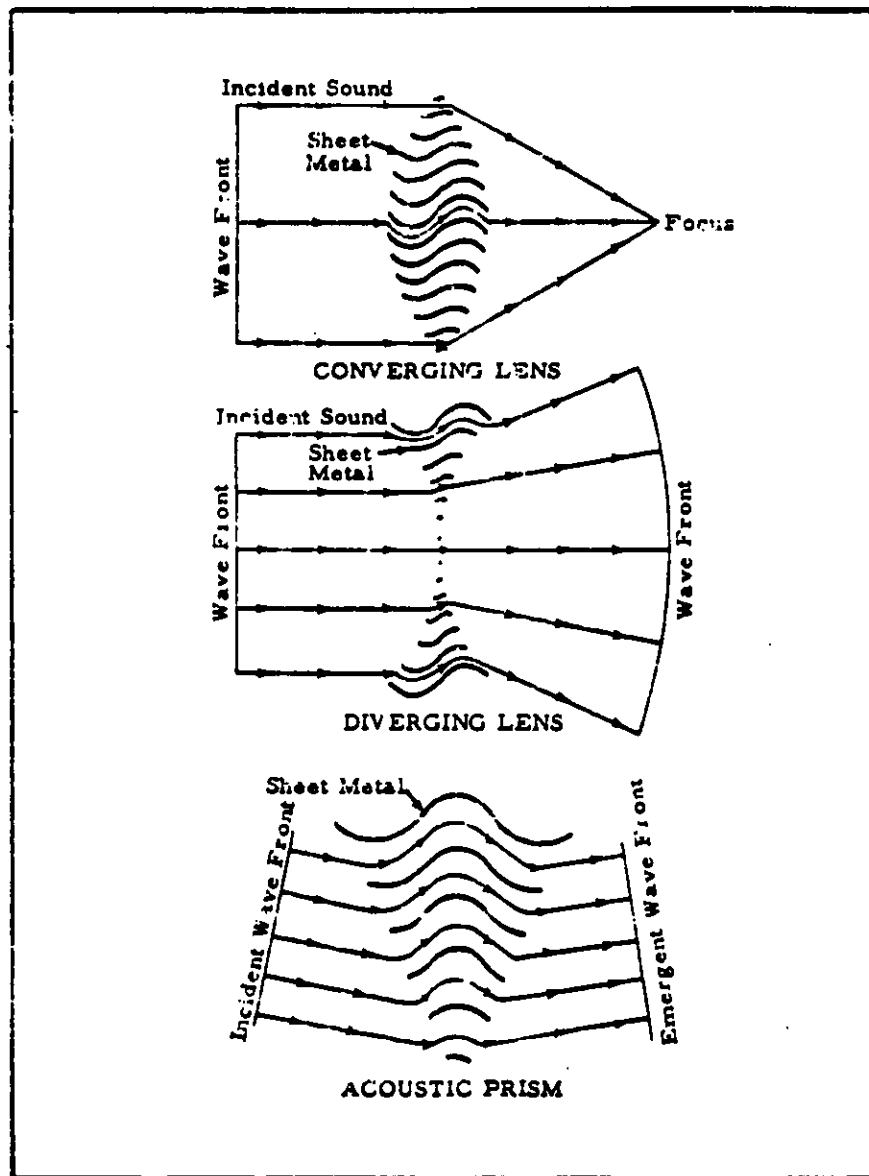
Figure 9.1.14 - Acoustic Lenses and Prism. 2
