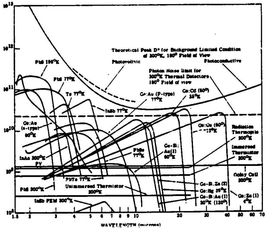
Figure 7.7.1b - Detectivity of Single-Element Detectors for the Spectral-Region between 1.5 and 70 Microns. (Compiled by Institute of Science and Technology, University of Michigan).
