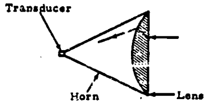
Figure 9.1.15 - Slant-Plate-Lens-Horn Microphone.
