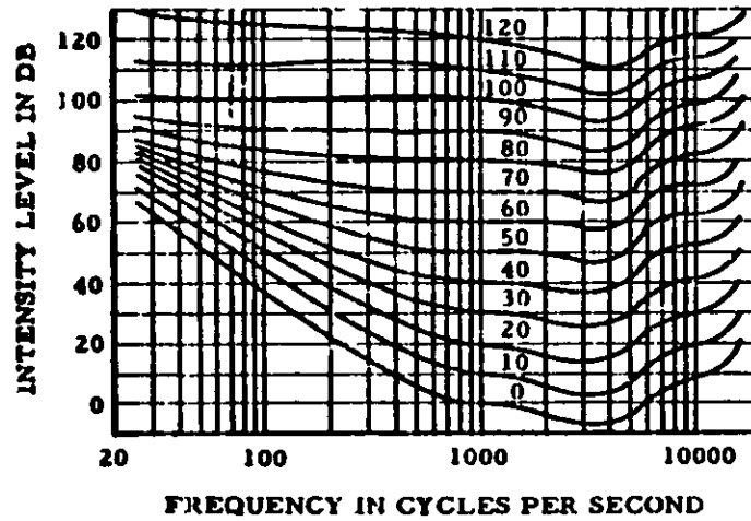
Figure 9.1.1 - Contour lines of equal loudness for normal ears. Numbers on curves indicate loudness level in phons. 0 db = 16^{-16} watts per square centimeter. 0 db = 0.000204 dyne per square centimeter. (After Fletcher and Munson.)
