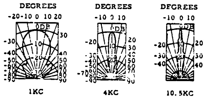
Figure 9.1.16 - Directional characteristics of a 29 inch diameter, 30 inch focal length slant-plate-lens-horn microphone.
