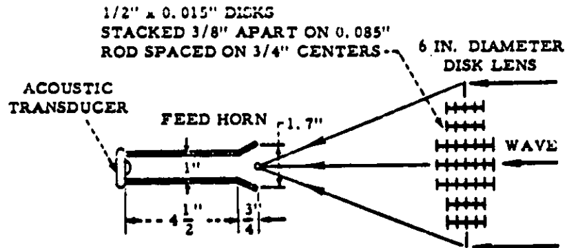
Figure 9.1.11 - Disk Lens for High Frequency Sound Collection.
